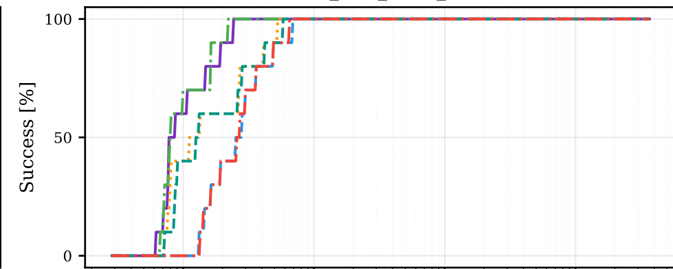
UR10_pick_place_drill
